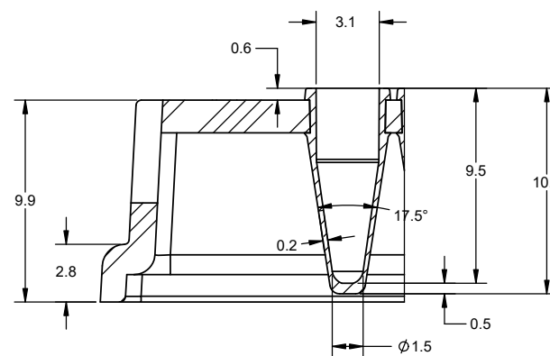
DETAIL W
